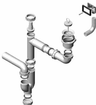
Waste kit 1XSP 70 - PP
