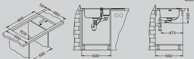
Strainer bowl stainless 1056616
