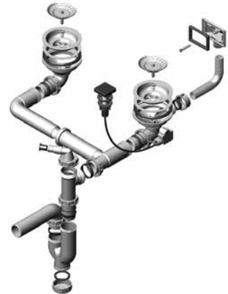
Waste kit 2XQM 114 - PP - 114 POP- UP
