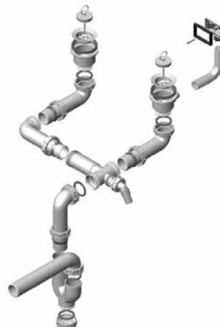
Waste kit 2XSP 70 - PP - 70
