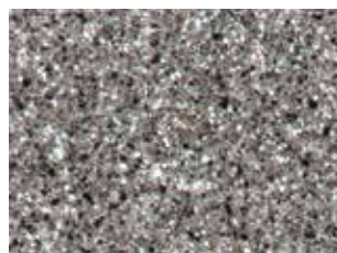
granulite 1055
